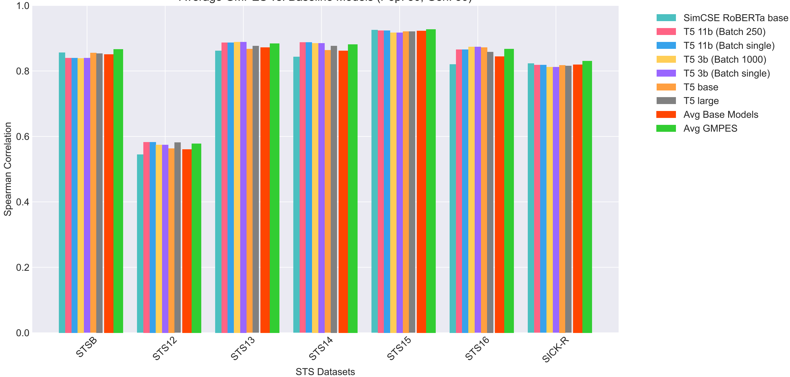
Average GMPES vs. Baseline Models (Pop: 50, Gen: 50)
